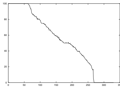
Fig. 5. Maximal CQTS value according to the user rank
